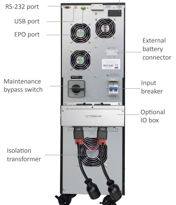
TX91 rear view
